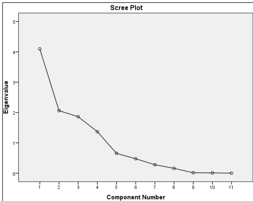
Fig 2: Scree Plot
