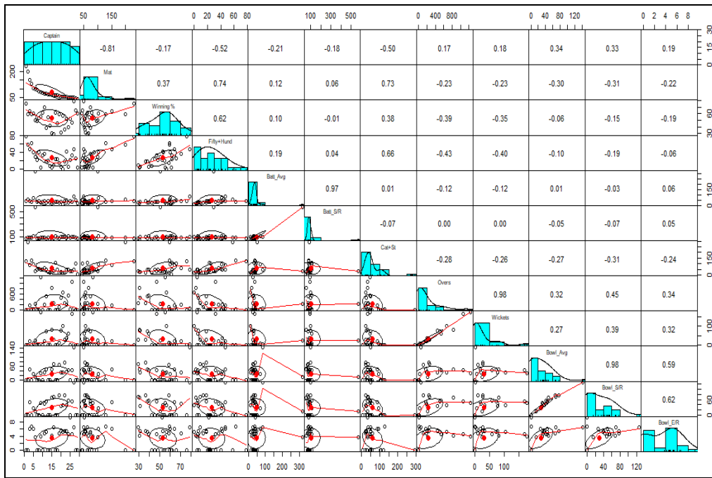
Fig 1: Sample Correlation Matrix for 29 Captains
