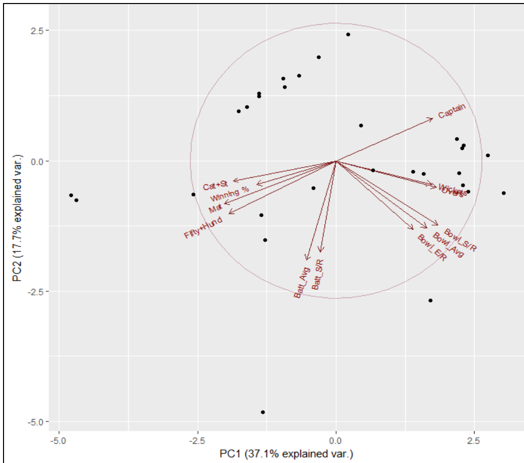
Fig 3: Loading Plot
